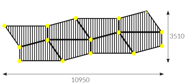
15 Masten / 8 Dachpanele
