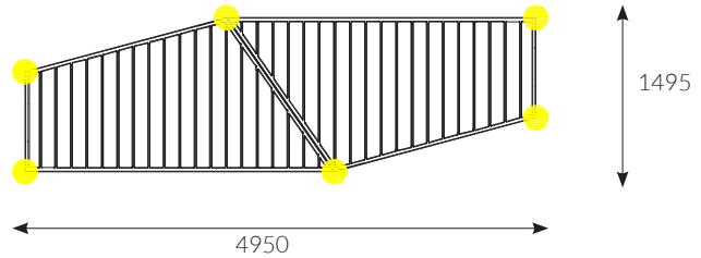
6 Masten / 2 Dachpanele
