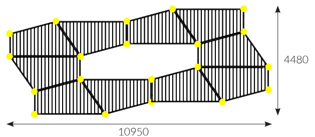
20 Masten / 10 Dachpanele
