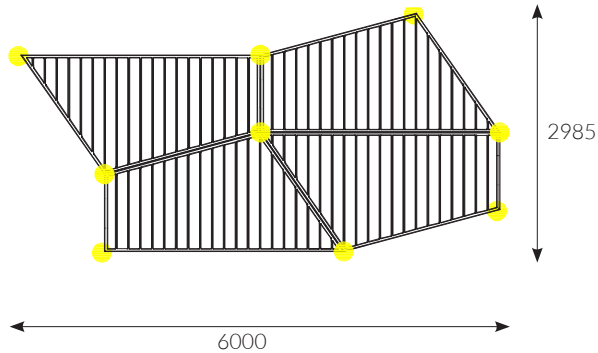
9 Masten / 4 Dachpanele
