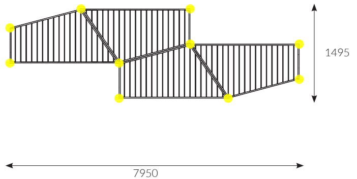
10 Masten / 4 Dachpanele
