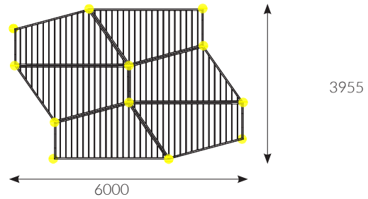
12 Masten / 6 Dachpanele
