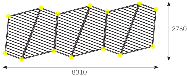
14 Masten / 6 Dachpanele
